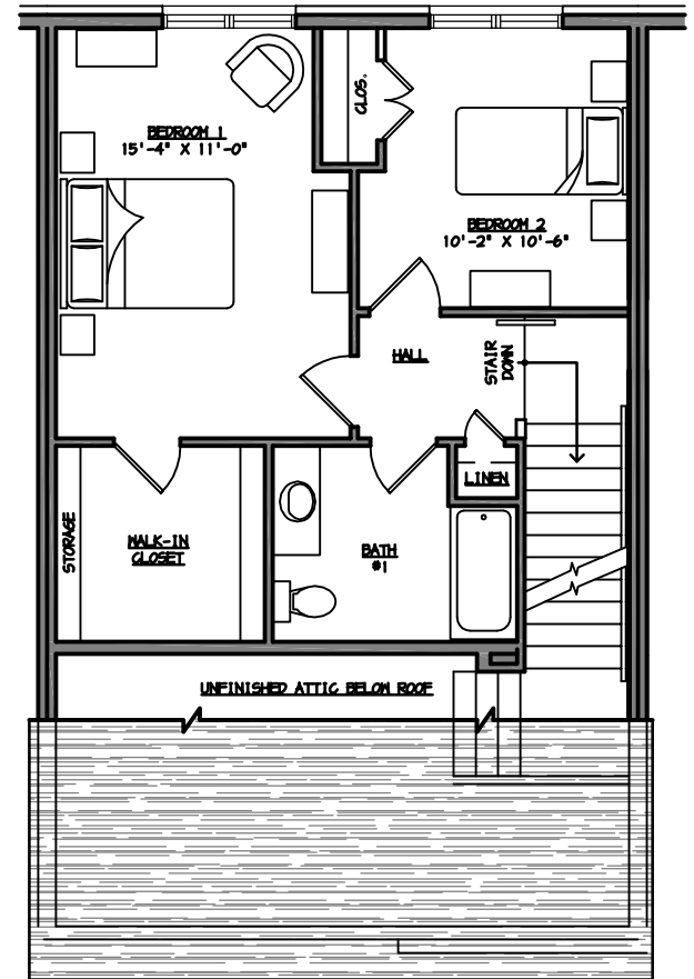
THIRD FLOOR
