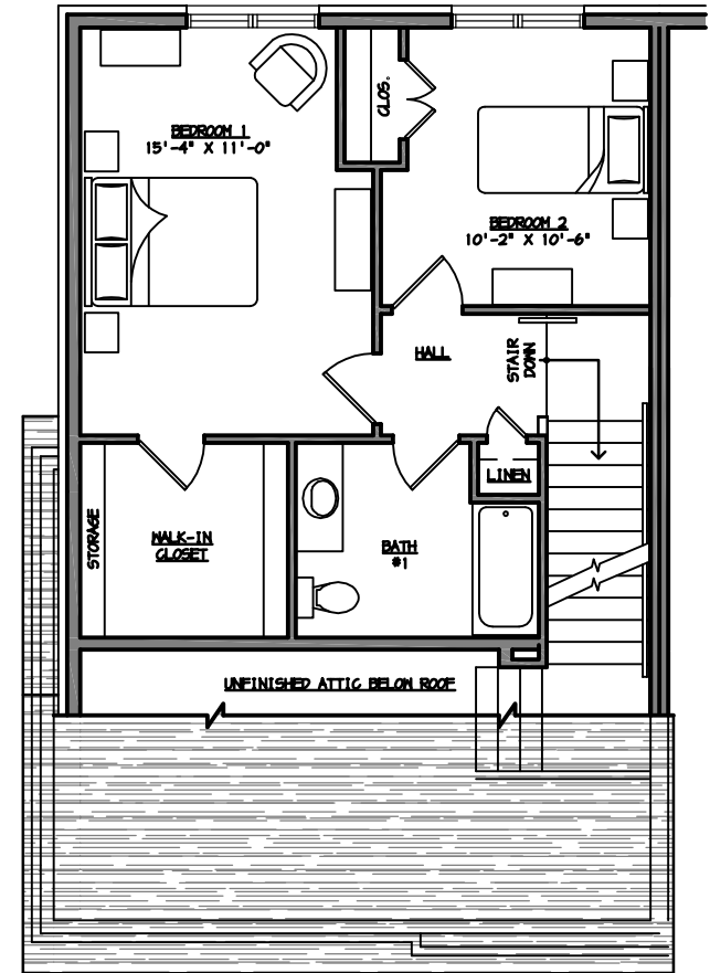
THIRD FLOOR
